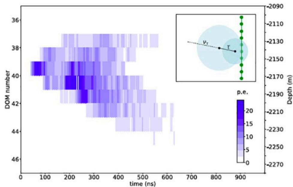
The IceCube Neutrino Observatory has detected seven astrophysical tau neutrinos. The once-elusive particles are weakly interacting, can travel astronomical distances unscathed, and can be traced back to their sources, potentially revealing the mysteries of their cosmic origins. Image shows the light signal of one of the energetic astrophysical tau neutrinos detected by multiple photosensors in the IceCube Neutrino Observatory at the South Pole. Credit: IceCube Collaboration
